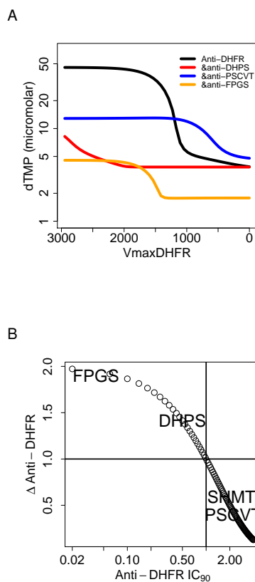
Fig. 5 Predicting synergistic combinations of antifolates. (A) The values for the V_{max} of DHFR were scanned against negligible V_{max} values (0.01) of other enzymes included in the model. The trends observed here are logarithmic. (B) Describing the effect of inhibiting other enzymes on the ICs for anti-DHFR inhibitors. The X-axis is logarithmic and represents an hypothetical scale of the IC_{90} values for an inhibitor of DHFR on its own (unity) or in the presence of another compound (values below, equal or above 1.0). Y-axis represents the difference between of the IC_{90} for an anti-DHFR alone minus the IC_{90} of the same anti-DHFR when in the presence of another compound. This difference is used as exponential of 2 as numeric base (see main text).
