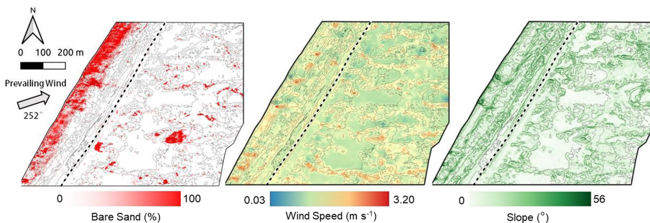
Fig. 4 2.5 m 2 resolution grid squares of bare sand percentage, wind speed (0.4 m above the surface) and dune slope at Ainsdale. The dashed line represents the frontal-hinterdune boundary. Contours are at 2 m intervals. The bare sand classification map represents the first replicate of three
