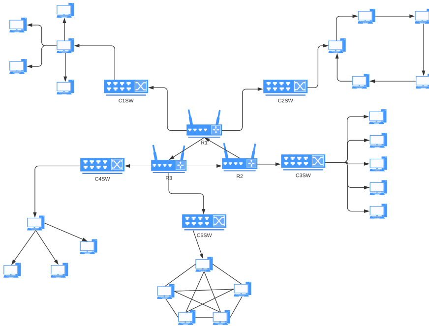
Figure 3: Network with 5 Nodes per Cluster configuration
