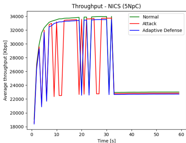
Figure 15: Adaptive Defense Performance with 5NpC
