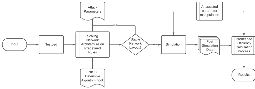
Figure 2: Flow diagram of testbed
