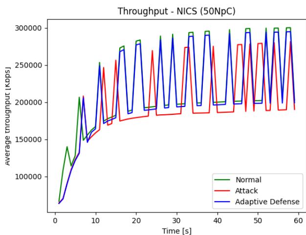
Figure 17: Adaptive Defense Performance with 50 Nodes per Cluster
