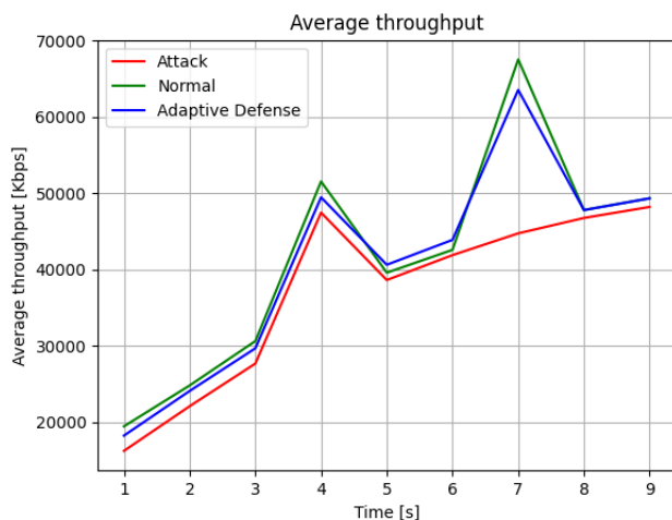
Figure 18: Case2: Adaptive Defense Performance with 5 Nodes per Cluster
