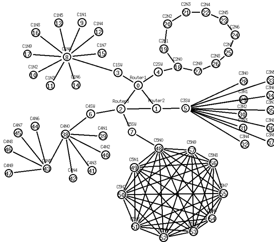
Figure 4: Network with 10 Node per Cluster configuration
