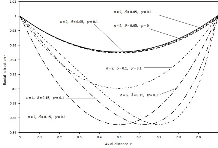
Figure 2: Shape of artery for different values of n , \delta and \psi
