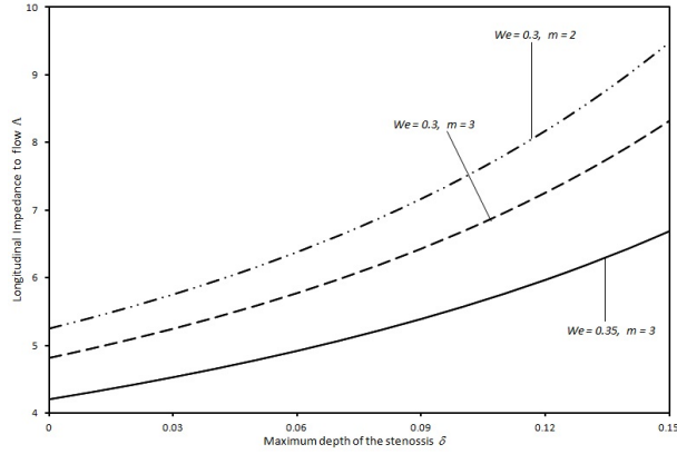
Figure 8: Variation of longitudinal impedance to flow with the maximum depth of the stenosis for different values of We , m and \psi with Q = 0.3 , A = \alpha = 0.2 , n = 2 , \psi = 0.1^\circ and t = 60^\circ .
