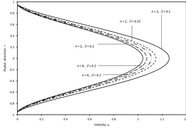
Figure 3: Velocity distribution for different values of n and \delta with Q = We = 0.3 , t = 45^\circ , \alpha = 0.2 , z = 0.5 , \psi = -0.1^\circ and A = 0.2 .
