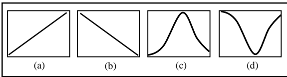
Fig. 4. Four primitive patterns: (a) Linear rise, (b) Linear fall, (c) Gaussian Bell curve, (d) Inverted Gaussian curve
