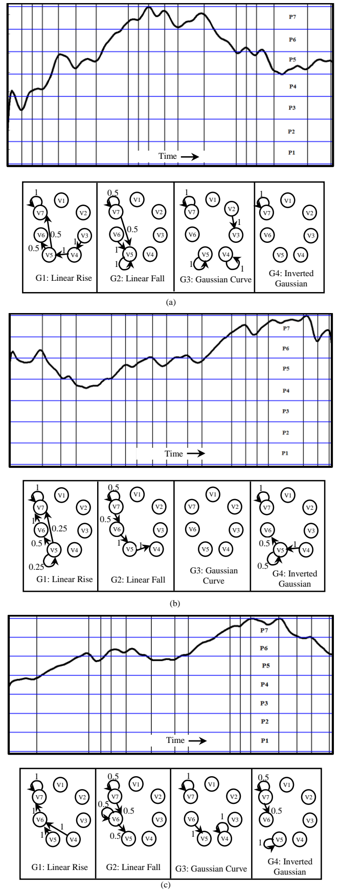
Fig. 7. Predictor graphs obtained from segmented TAIEX close-price time-series for the years (a) 1991, (b) 1994, (c) 1997. The entire TAIEX time-series is partitioned into intervals P1 to P7 (shown by horizontal lines), and the close-price series for each year is separately segmented where the segment boundaries are shown by vertical lines.
