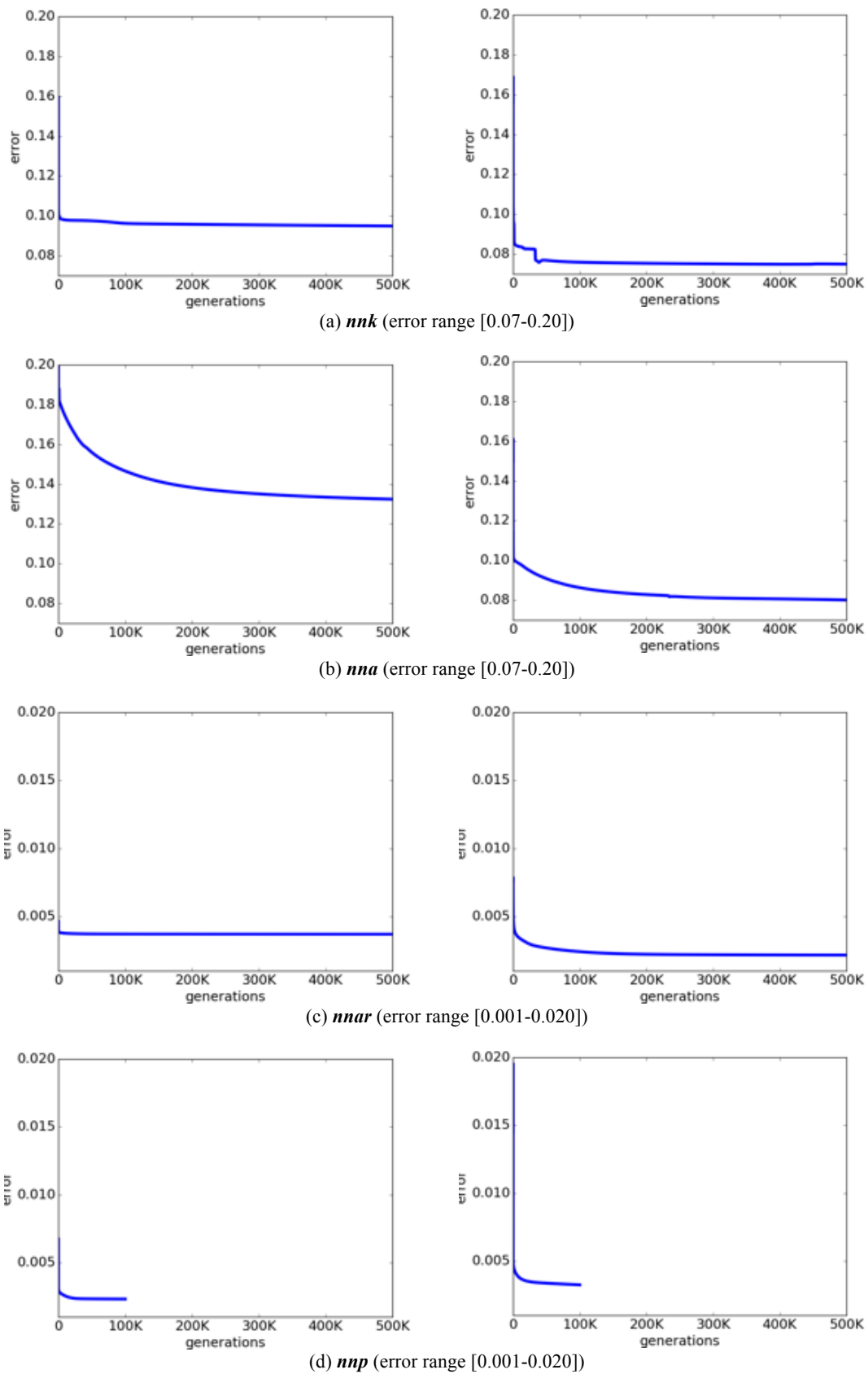
Fig. 8. Improvement in error during training. The x-axis starts at 0 and extends for 500 K generations (except in the case of the nnp model, where training was completed after 100 K generations). The y-axis contains the error rate, as labelled. See text for details.
