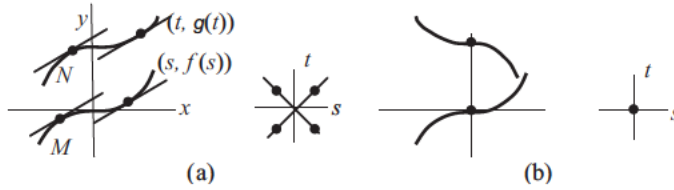
Fig. 2. Two inflexions with parallel tangents, (a) with the same orientations, that is f''(0)g''(0) > 0 , and (b) with opposite orientations, that is f''(0)g''(0) < 0 . In (a) there are sets of four nearby points all with parallel tangents, while in (b) there is no pair with parallel tangents apart from those at the inflexions. The (s, t) diagrams represent pairs (s, t) giving parallel tangents.
