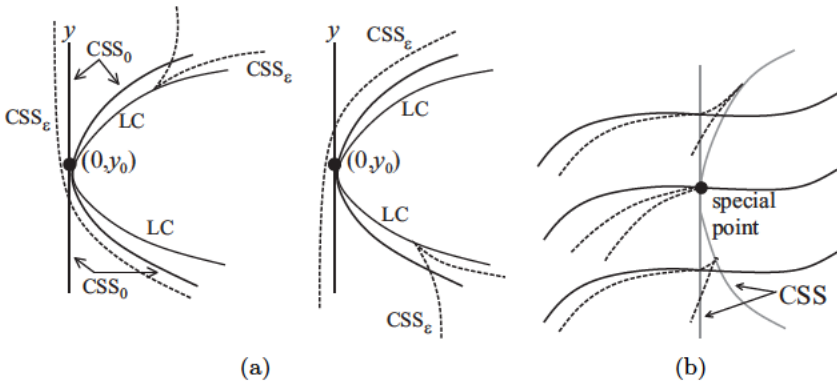
Fig. 5. The case \varepsilon = 0 . (a) The thick solid lines, marked CSS_0 , are the part close to a special point (0, y_0) of the CSS for \varepsilon = 0 , that is for two curves with parallel tangents at inflexion points. The thin solid line marked LC is the locus of cusps on the CSS for \varepsilon close to 0. The dashed line, marked CSS_\varepsilon , is the CSS itself for \varepsilon close to 0; one diagram will be for \varepsilon > 0 and the other for \varepsilon < 0 . Compare Figure 4. In (b) equidistants are drawn for \lambda at, and close to, a special point. The CSS is drawn in a lighter colour and the two “branches” of the equidistants are solid and dashed lines. At the special value one branch has a rhamphoid cusp.
