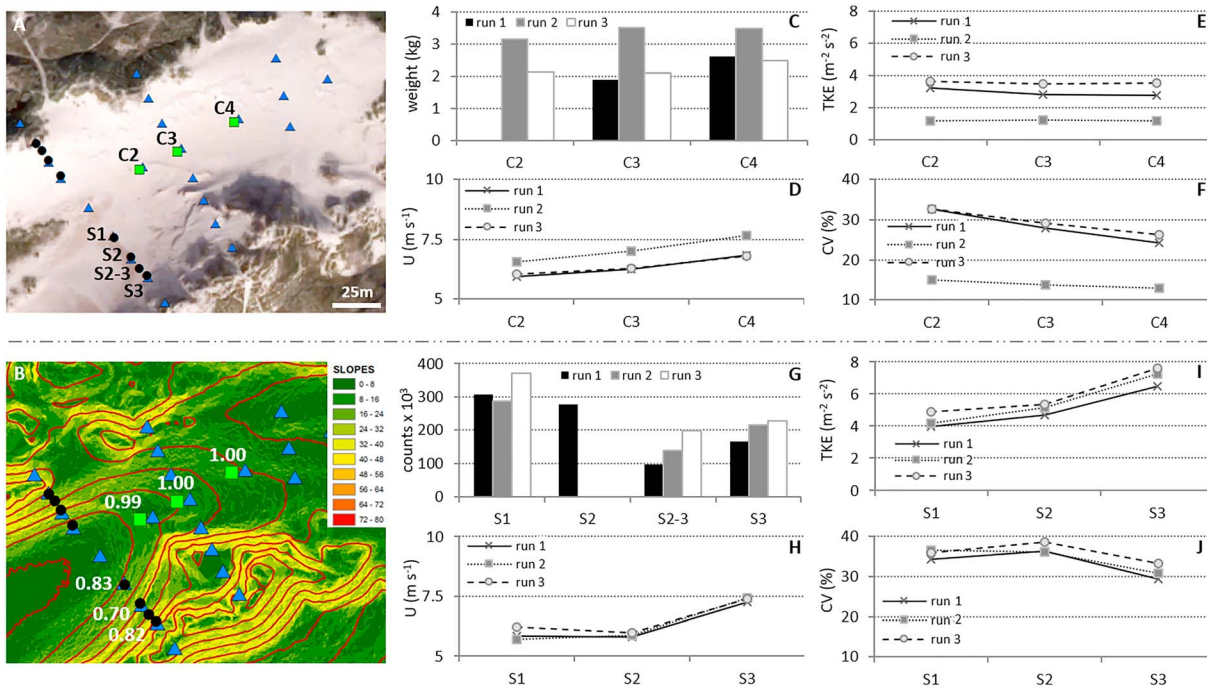
Figure 6. Spatial patterns of sand transport for all runs. (a, b) Transport sampling locations and 2-m slope contours at the study site, including run 2 activity parameter values in white (except for S2 due to instrument malfunctioning). (c–f) Total transport (kg) collected by the traps and average wind variables at colocated ultrasonic anemometers. (g–j) Total counts recorded by Laser Particle Counters and average wind variables at colocated ultrasonic anemometers. Run durations limited to 14 min for comparison purposes. CV = coefficient of variation; TKE = turbulent kinetic energy.
