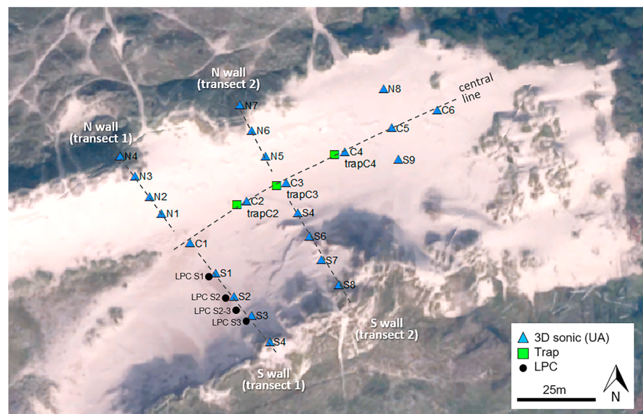
Figure 2. Grid of 3-D ultrasonic anemometers along the central line (C1 to C6), N wall (N1 to N7), S wall (S1 to S8), and toward the lobe (N8 to S9). Traps and Laser Particle Counters (LPCs) were collocated by ultrasonic anemometers (UAs) along the central line and transect 1.
