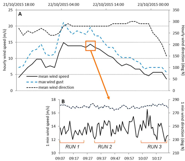
Figure 4. (a) Hourly wind data collected by a meteorological station in Crosby. Event lasted from the evening of the 21 October to midnight on the 22 October 2015. (b) Wind conditions measured by the 2-D sonic anemometer at the entry of the blowout during runs 1–3, during which transport was well developed throughout the dune landform.
