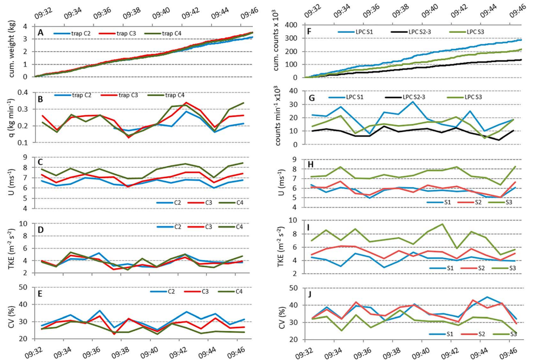
Figure 7. Temporal patterns of sand transport during run 2 for traps and colocated ultrasonic anemometers (a–e) and Laser Particle Counter and colocated ultrasonic anemometers (f–j). Cumulative weight (a) and counts (f) are displayed every 1 s. The remaining of the data are 1-min averages. Q = transport; U = wind speed; TKE = turbulent kinetic energy; CV = wind coefficient of variation.
