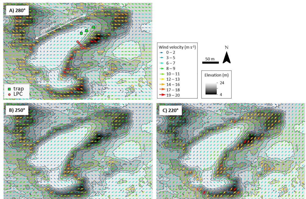
Figure 12. Simulated airflow patterns for three incident wind directions representative of wind events at the Devil's Hole. Wind flow was calculated using Reynolds-averaged Navier-Stokes equations in the computational fluid dynamics tool OpenFOAM. Wind vectors show near-surface (1 m above the underlying terrain) airflow at 10-m intervals. Elevation contours are spaced at 2-m intervals. The location of LPCs and traps has been included to allow for comparisons with Figures 5, 6, and 9. LPC = Laser Particle Counter.
