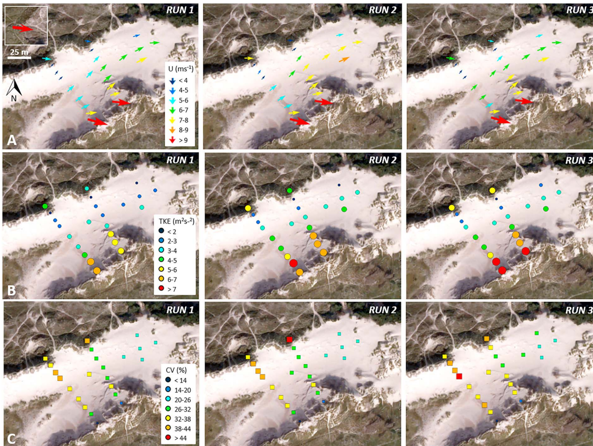
Figure 5. Average values recorded by the grid of ultrasonic anemometers (magnitudes indicated by both color and symbol size). (a) Wind speed ( U ) and direction. (b) Turbulent kinetic energy (TKE). (c) Coefficient of variation (CV). Input winds at the entry point of the blowout (inset in run 1) were steady from the W during the three runs (Figure 4).
