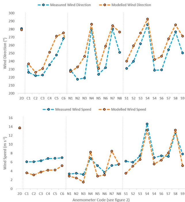
Figure 11. Measured and modeled wind direction and wind speed arranged by location within the deflation basin. Anemometer codes along the x axis refer to those presented in Figure 2.
