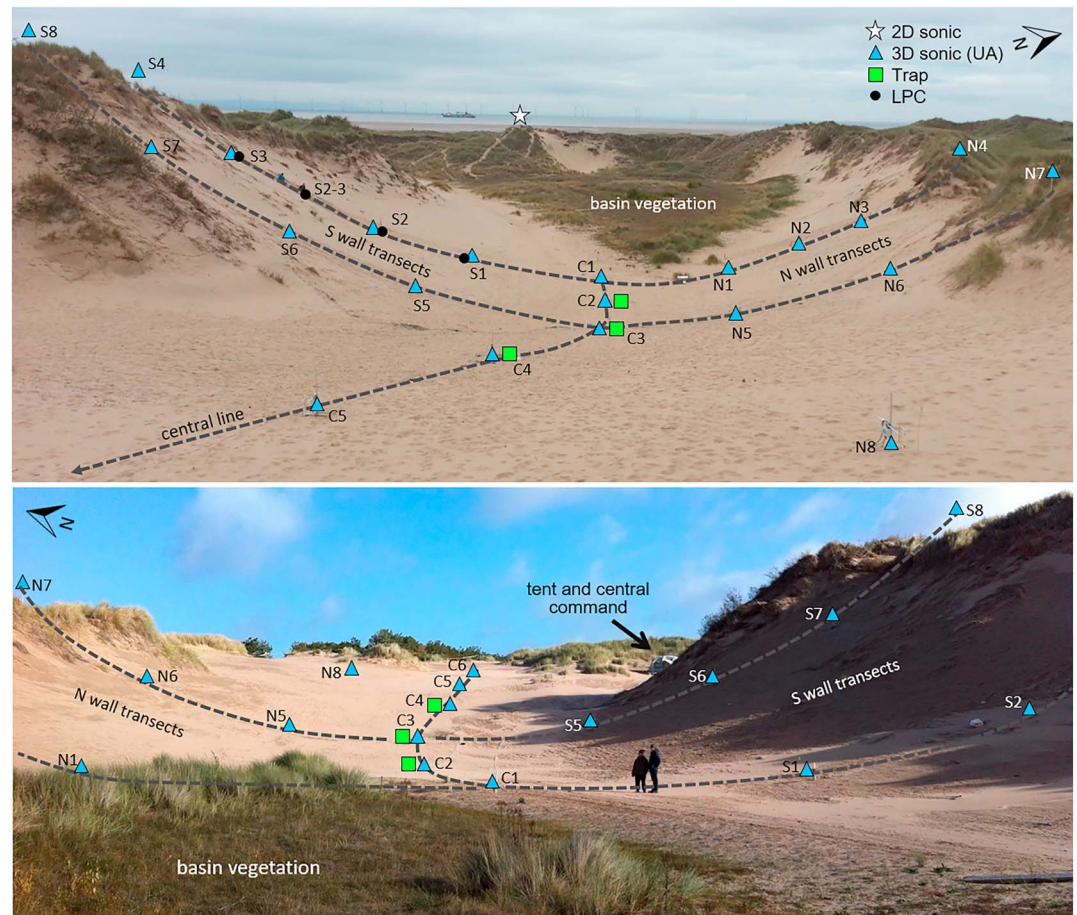
Figure 3. Seaward (above) and landward (below) views of the Devil's Hole and instrument grid. LPC = Laser Particle Counter; UA = ultrasonic anemometer.
