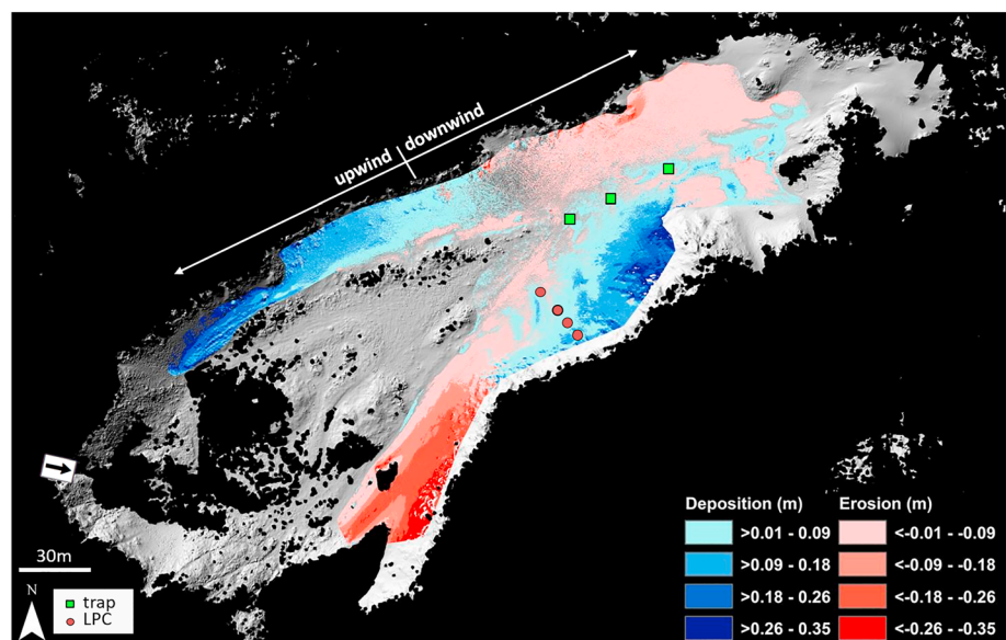
Figure 9. Short-term elevation changes calculated by comparing the preevent and postevent TLS scan. Areas in black indicate no data collected, and areas in gray were excluded from the analysis because of poor data quality or missing values in one of the scans. LPC = Laser Particle Counter.
