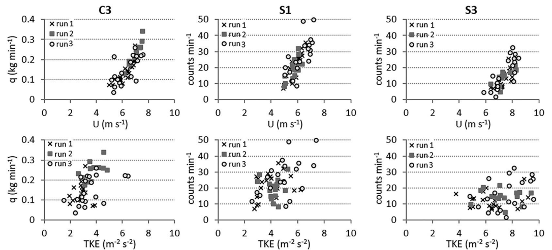
Figure 8. Scatter diagrams for transport versus wind speed ( U ) or TKE at the basin ( q , measured by trap C3), lower slope of the south wall (LPC S1), and upper slope of the south wall (LPC S3). Correlation values for all relationships between transport and wind variables are presented in Table 3. TKE = turbulent kinetic energy.
