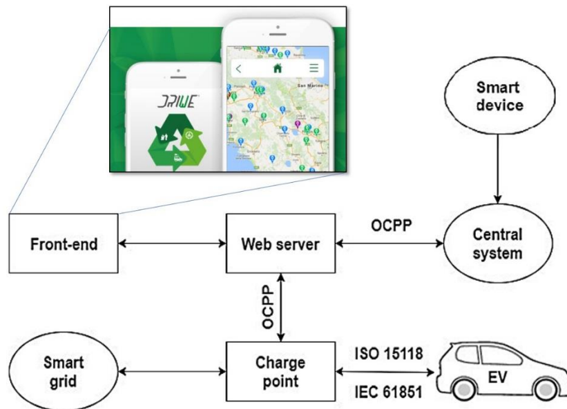
Figure 2. The main structure of the DRIWE operating scheme: on the end-user side, a mobile app allows accessing DRIWE services (and localizing geo-referenced charging points).
