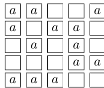
Fig. 2: The a -map of the array X
